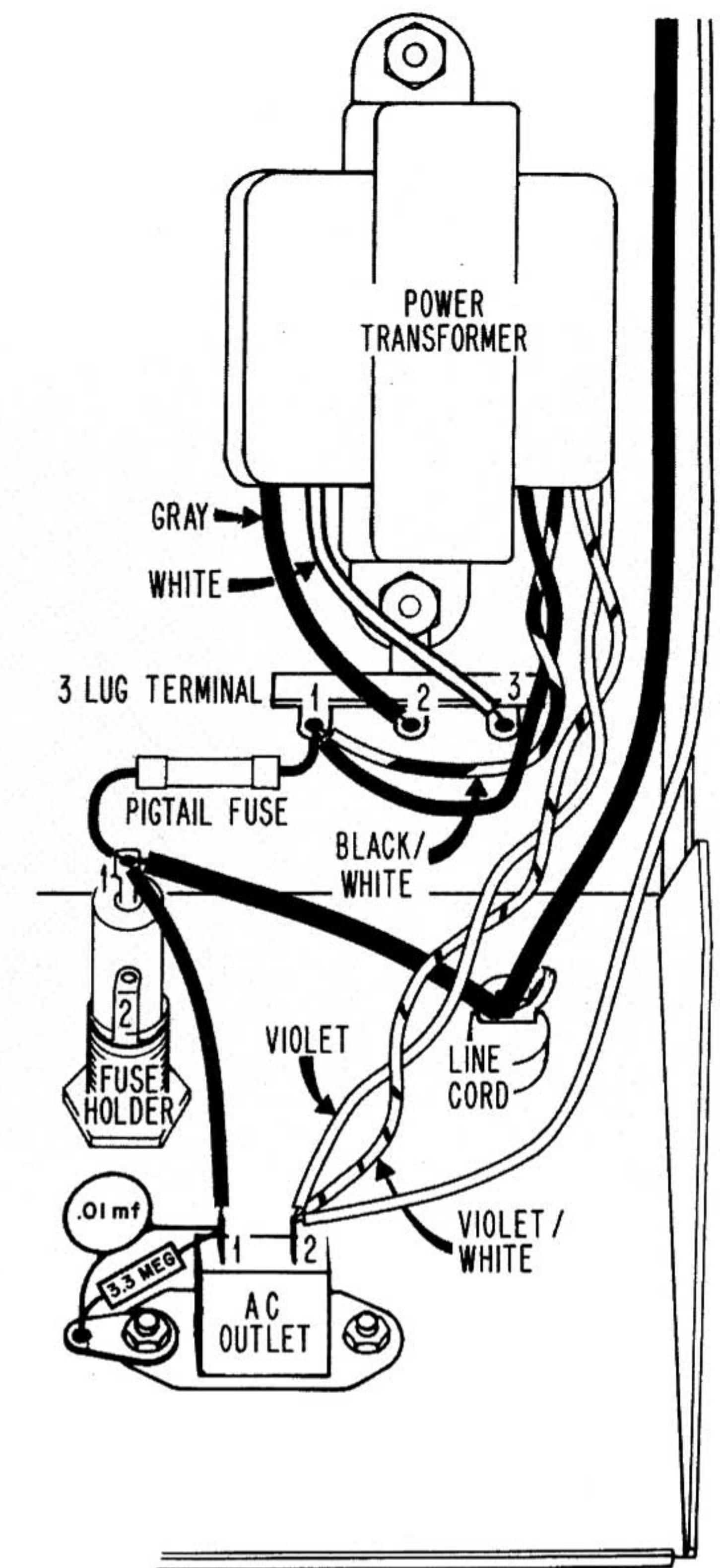
120 VOLT AC LINE WIRING FOR UNITS OBTAINED IN CANADA
